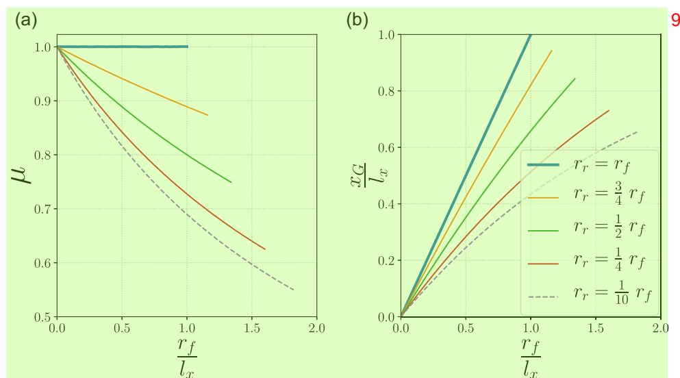
FIGURE 6 Minimum friction coefficient needed to climb a bilateral obstacle (step) with both front and rear wheels depending on their radius (a) and corresponding optimal position of the CoM in each case (b). The curves stop when front and rear wheels collide due to their side.
