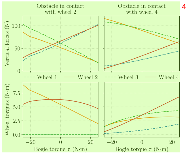
FIGURE 5 Distribution of the rover load and wheel torques depending on the internal torque \tau when dealing with a vertical obstacle blocking one of the front wheels or one of the rear wheels while \Delta x = 0 .
