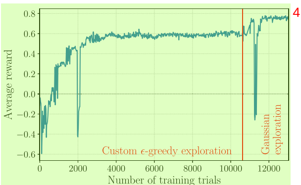
FIGURE 14 Evolution of the average reward per evaluation trial, that is, using the state of the networks at different stages of the training while omitting exploration.
