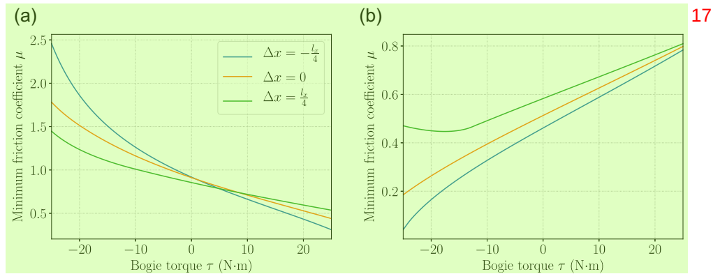
FIGURE 4 Minimum friction coefficient necessary to overcome a vertical obstacle blocking the front right wheel (a) or the rear right wheel (b). The curves corresponding to the obstacle placed in front of the left wheels, that is, wheels 1 and 3, are similar and can be obtained by symmetry around the vertical axis. \Delta x defines a relative variation of the wheel positions, as depicted in Figure 3a. (a) Obstacle in contact with wheel 2, and (b) obstacle in contact with wheel 4.
