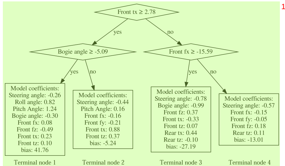
FIGURE 16 Linear model tree providing the steering angle rate control. 2
