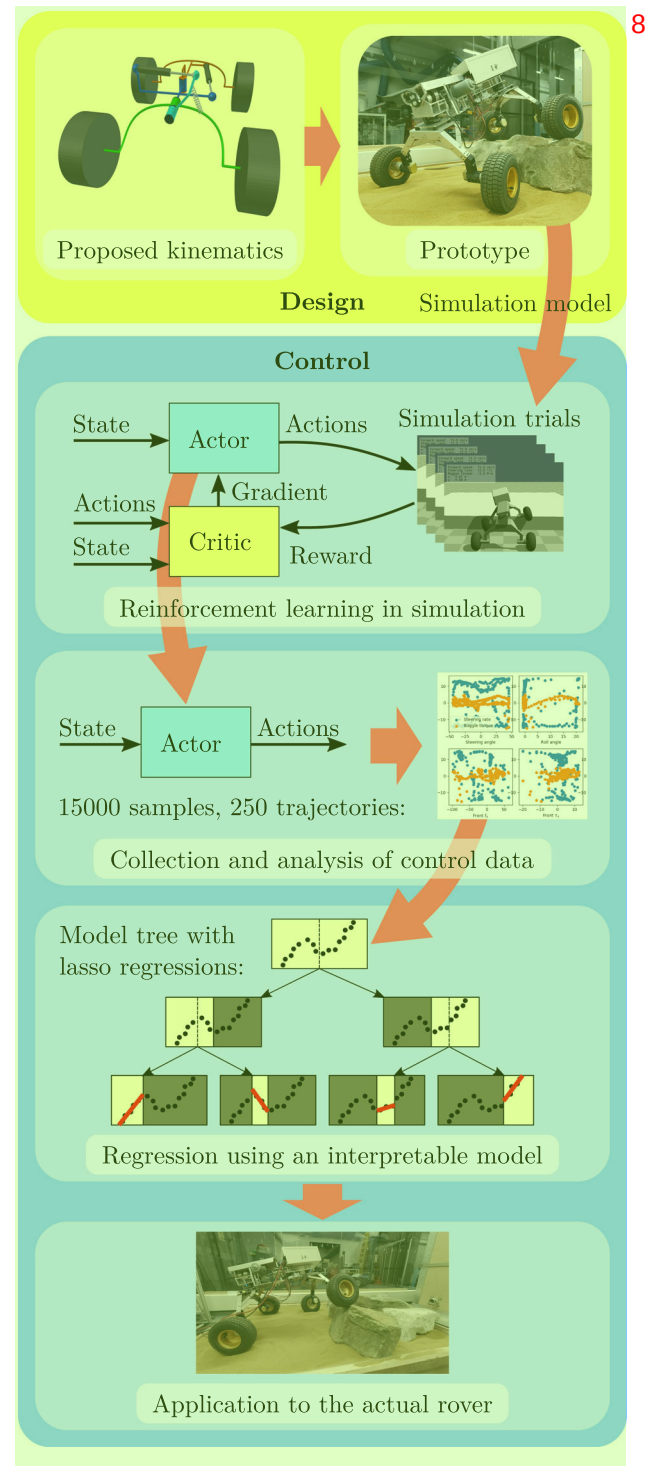
FIGURE 1 Summary of the methodology and contributions of the paper. From the proposed kinematic design, supported by static analysis, a prototype has been built. Based on the actual features of the prototype, a simulation model is used to train a neural network controller by reinforcement learning to leverage the actuated joints of the chassis to cross steep obstacles. The control outputs of the neural network controller are then collected and analyzed. The obtained input-output data are used to train a linear model tree to reproduce the outputs of the neural network in an interpretable way. The resulting controller is finally applied and tested on the actual prototype.
